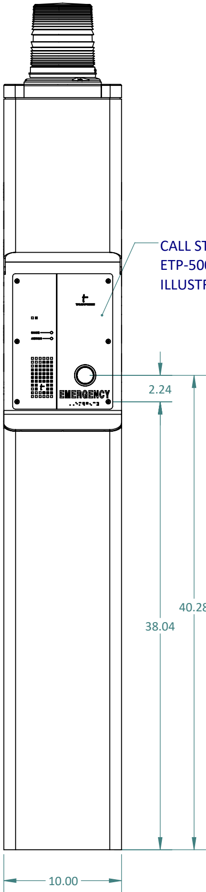
FRONT VIEW
