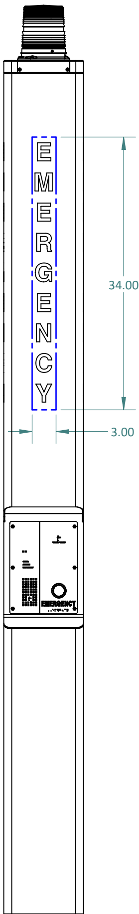
FRONT VIEW
