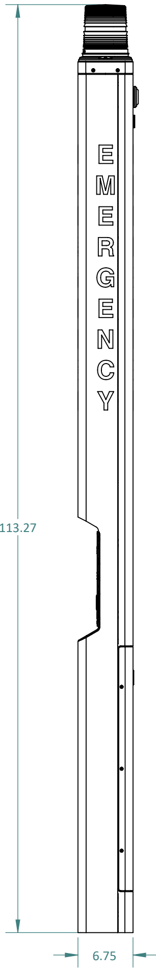
SIDE VIEW
