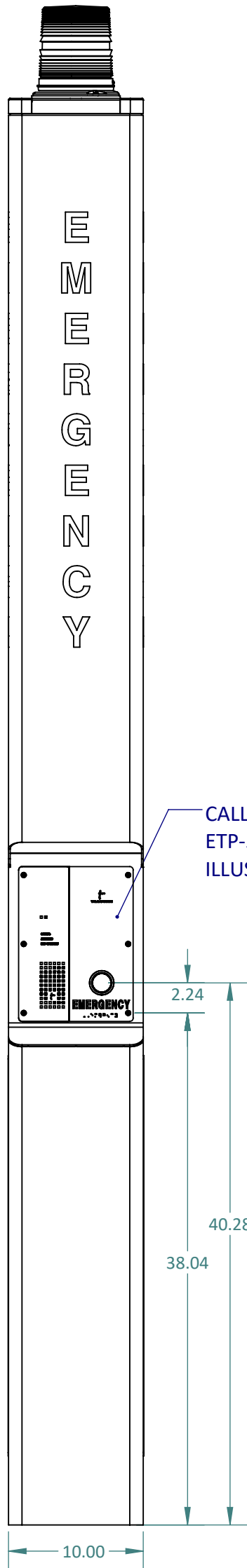
FRONT VIEW
