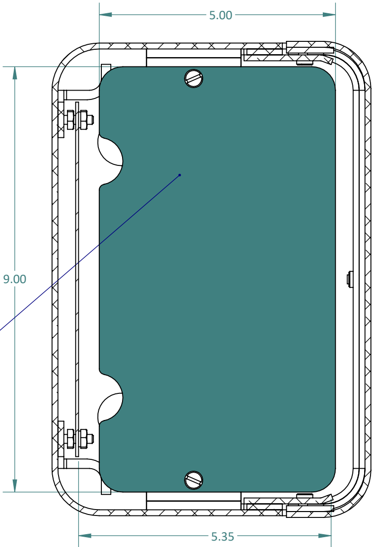
SECTION C-C SCALE 1 : 2
