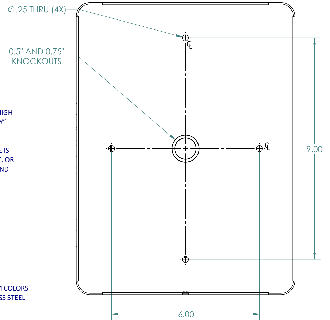
REAR VIEW
