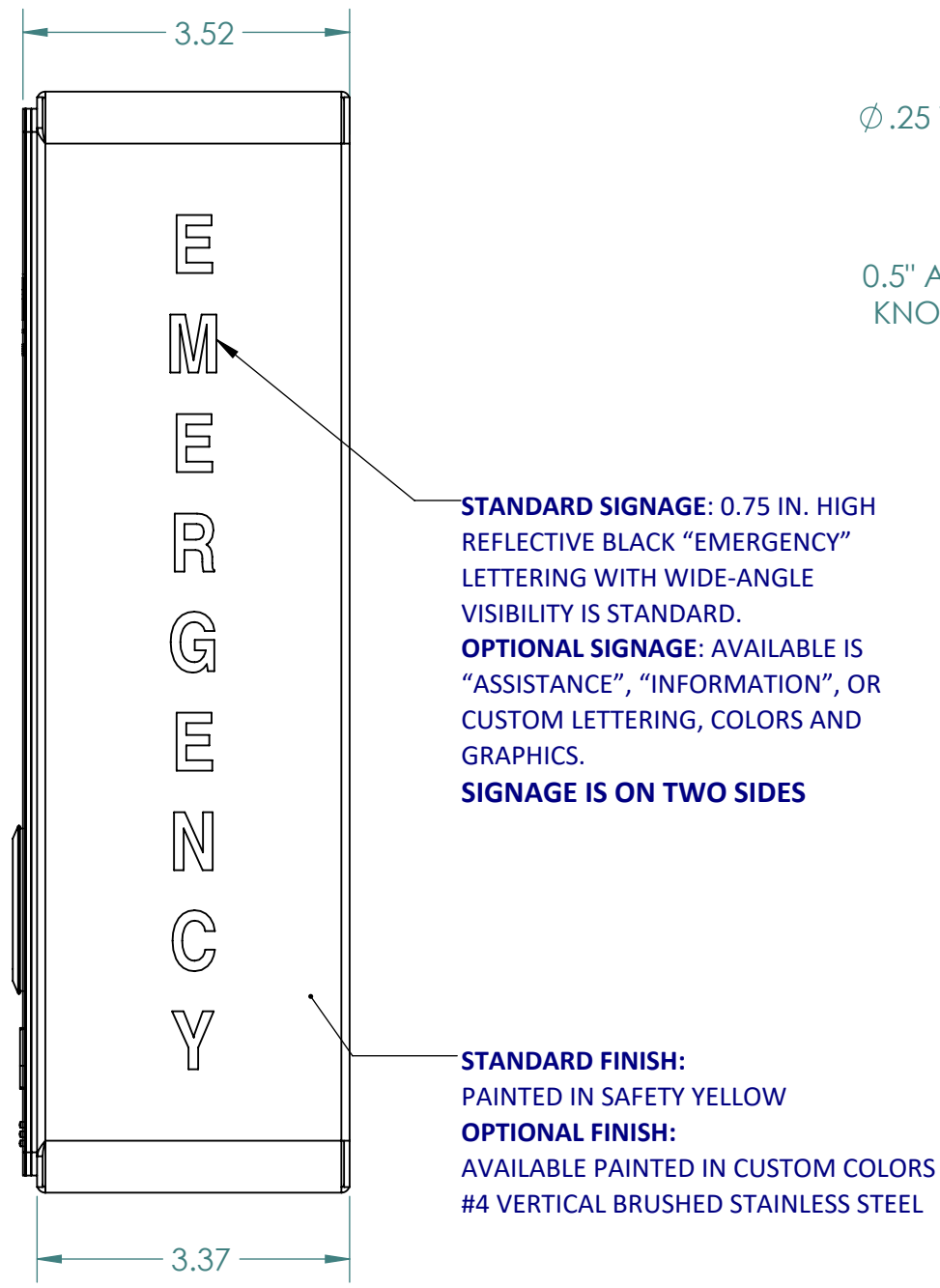
SIDE VIEW
