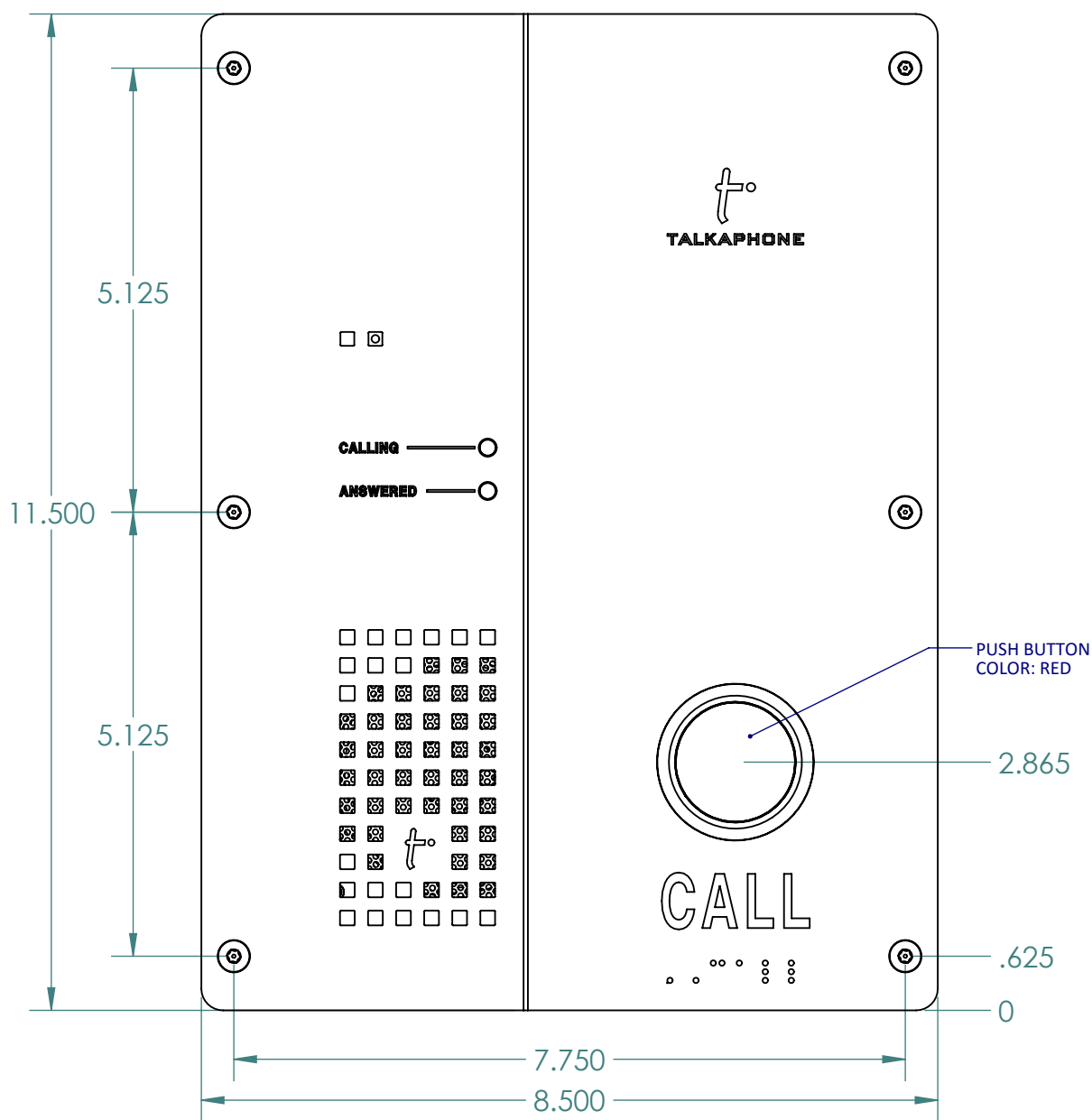
FRONT VIEW
