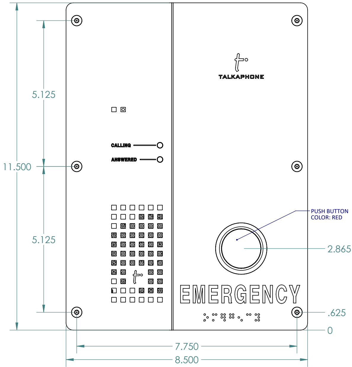
FRONT VIEW
