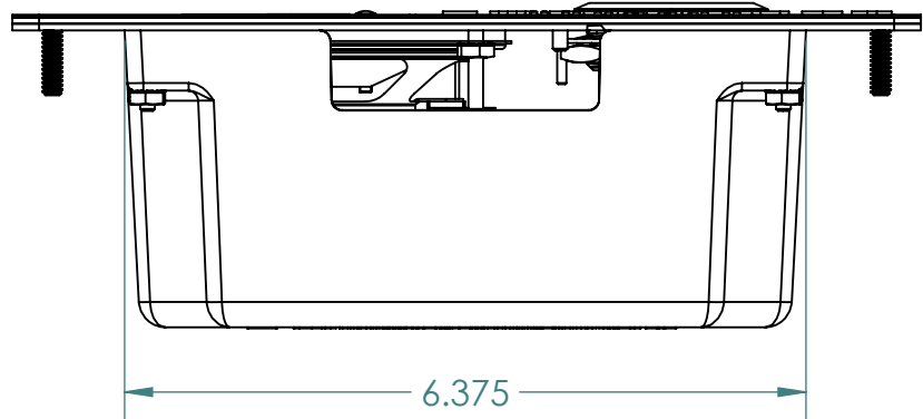
BOTTOM VIEW
