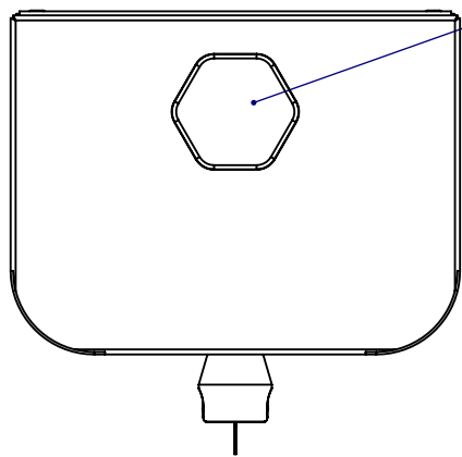
AERATOR (IP66 RATED) GORE PMF200542
