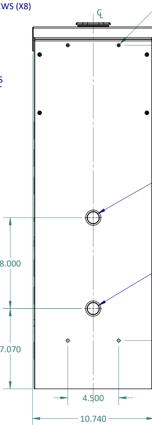
BOUNDING BOX DIMENSIONS FOR OPTIONAL SIGNAGE NOT PROVIDED BY TALKAPHONE: 21.00"H X 2.00"W
