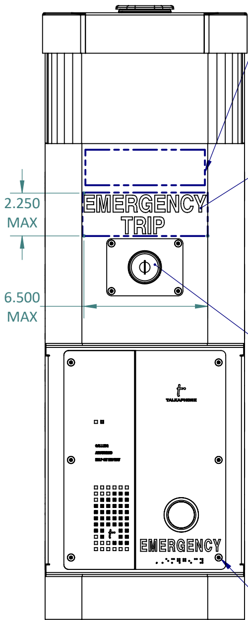
BOUNDING BOX DIMENSIONS FOR OPTIONAL SIGNAGE NOT PROVIDED BY TALKAPHONE: 2.125"H X 6.25"W
