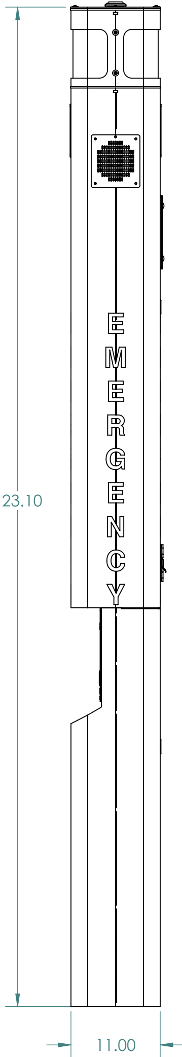
SIDE VIEW
