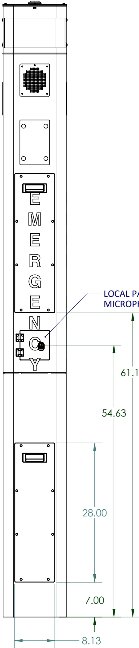
REAR VIEW
