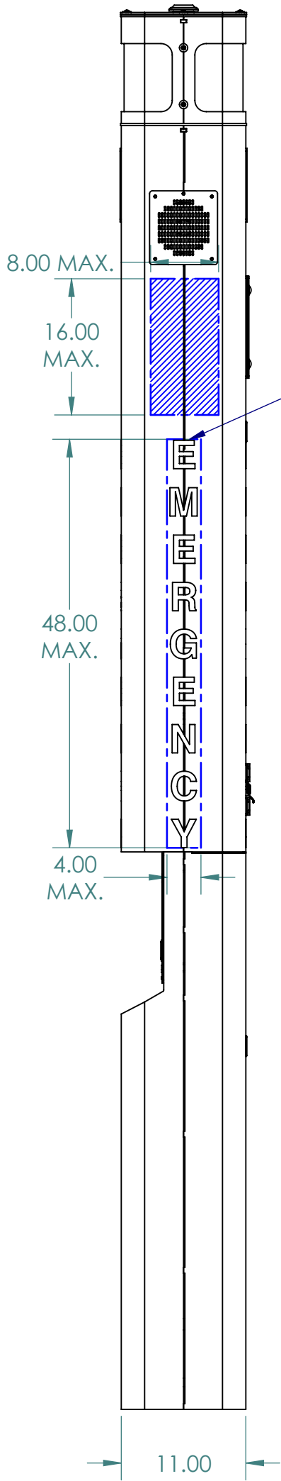
SIDE VIEW
