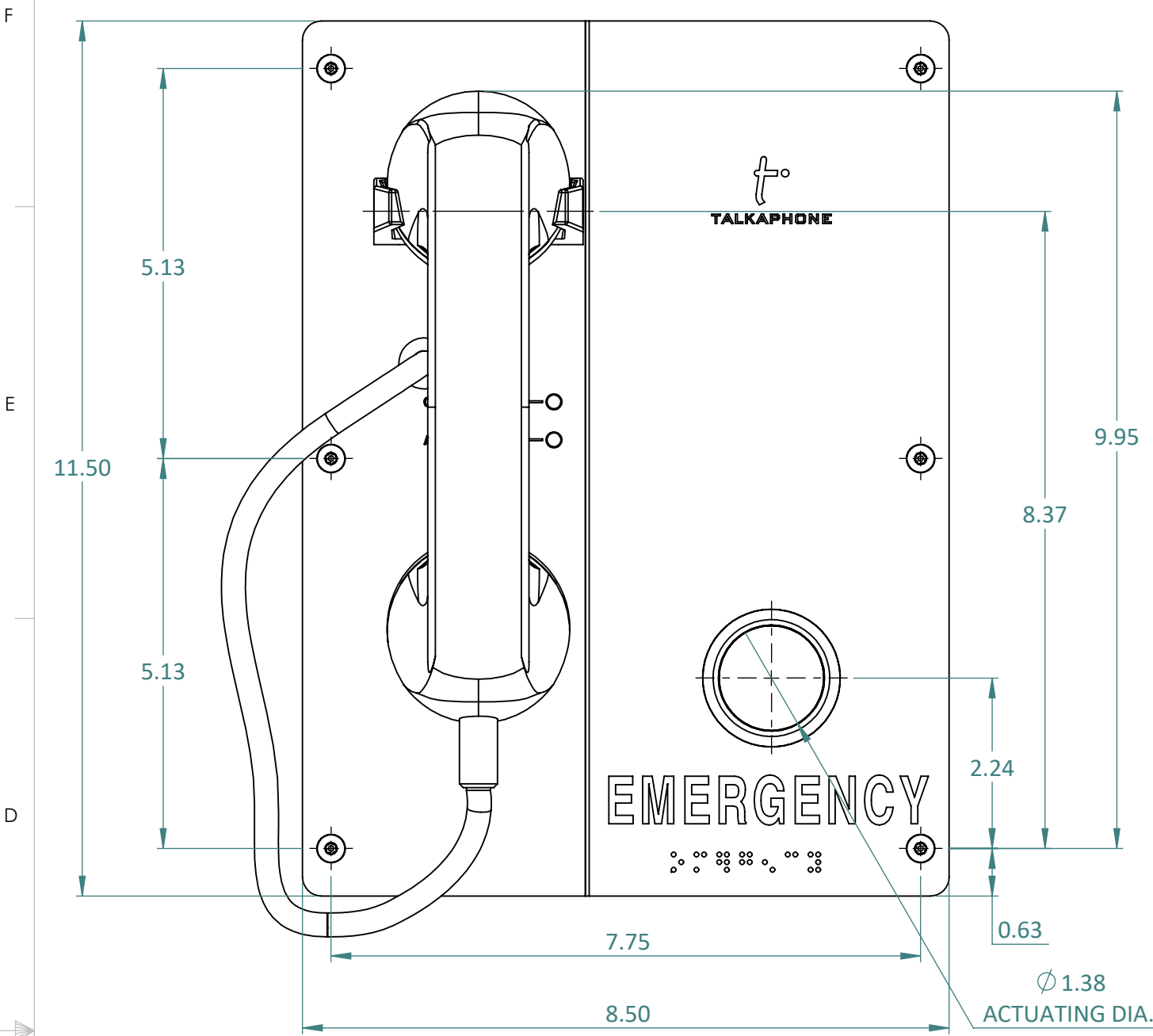
FRONT VIEW
