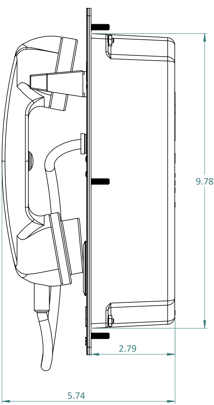
SIDE VIEW
