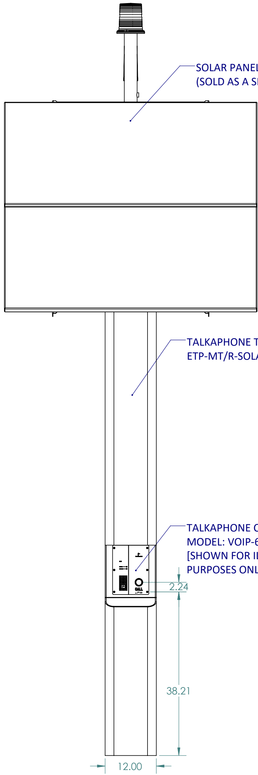
FRONT VIEW
