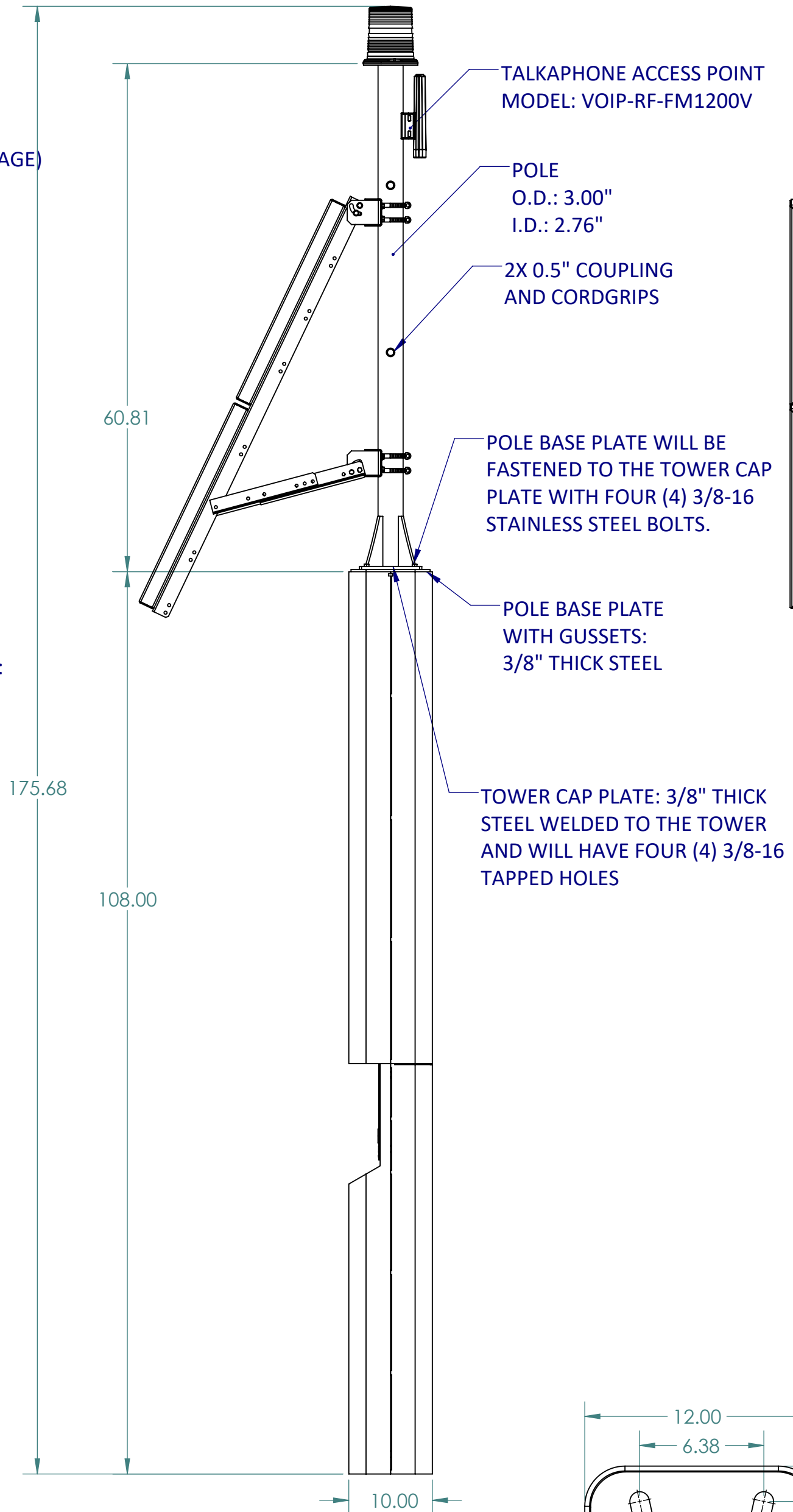
SIDE VIEW
