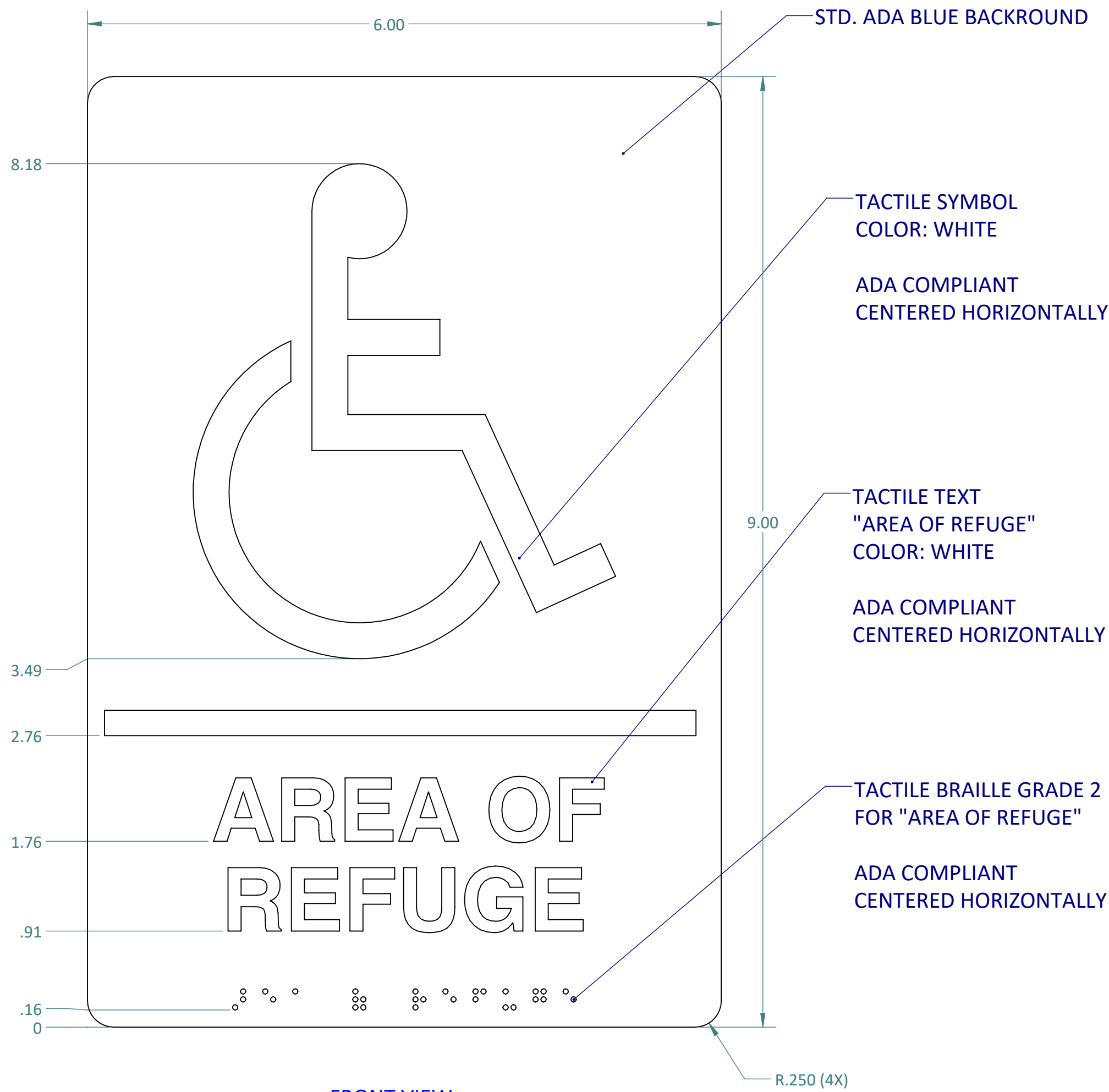
FRONT VIEW
