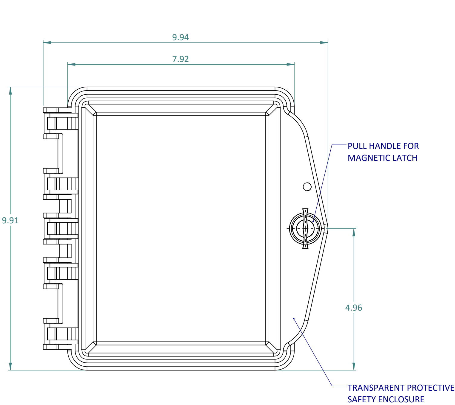
FRONT VIEW
