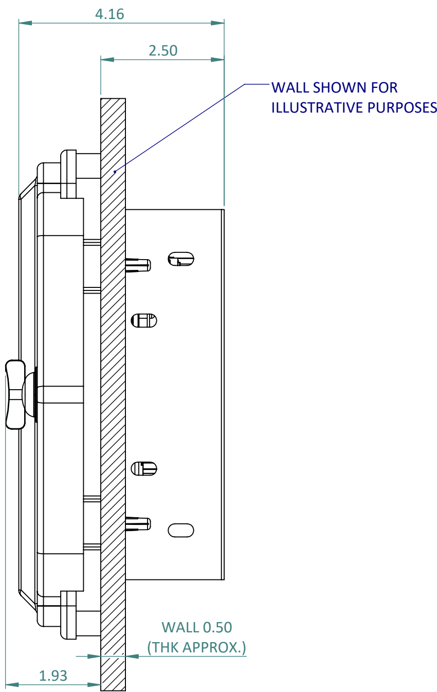
SIDE VIEW
