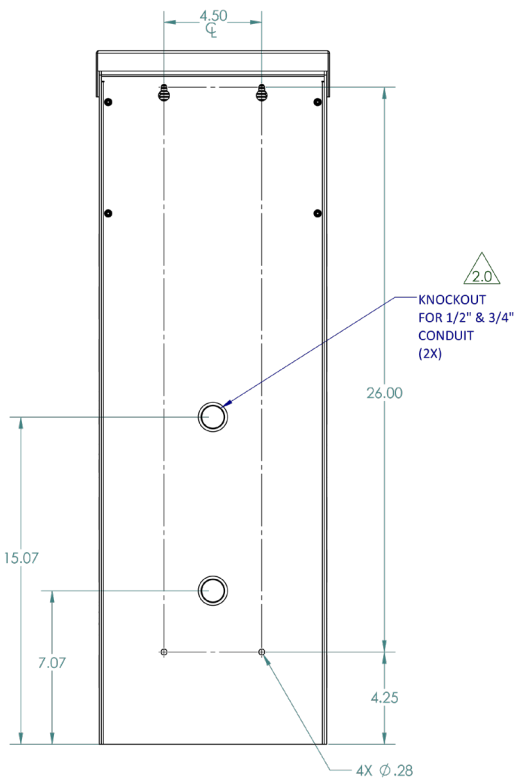
REAR VIEW
